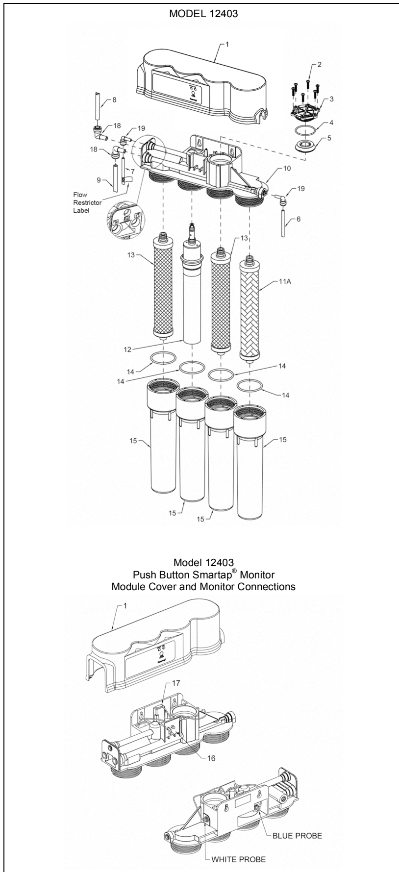
Figure 8: Exploded Schematic, 12403 Model Series
